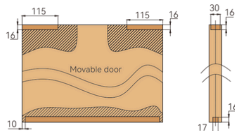
Hanging box size and door slotting requirement
