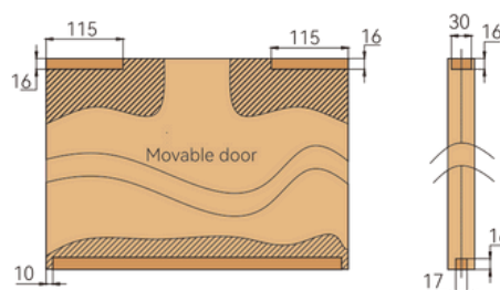
Hanging box size and door slotting requirement
