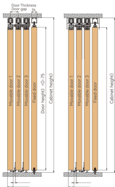
Single track diagram Connecting track diagram
