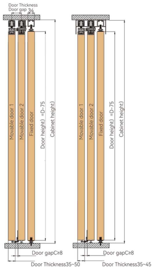
Single track diagram
