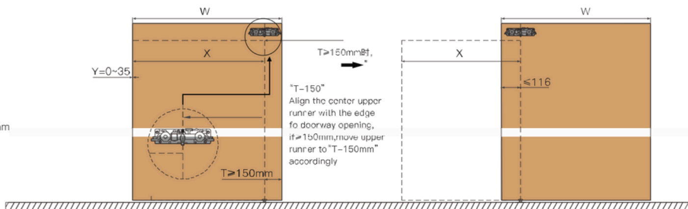
Damper installation size
