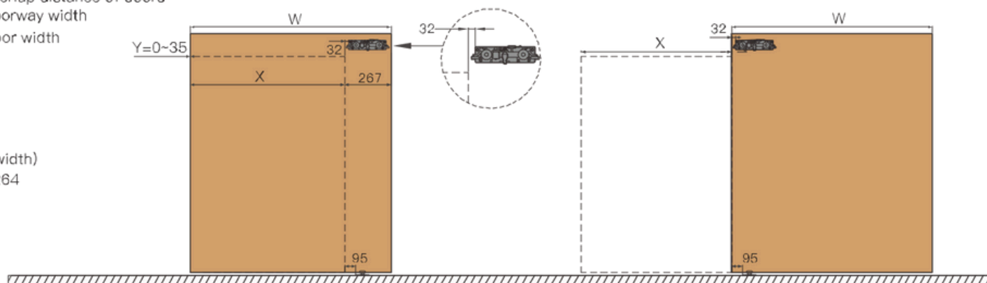
Damper installation size
