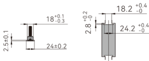
Hanging box size and door slotting requirement
