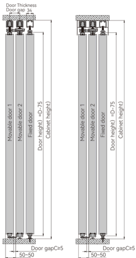
Single track diagram Connecting track diagram
